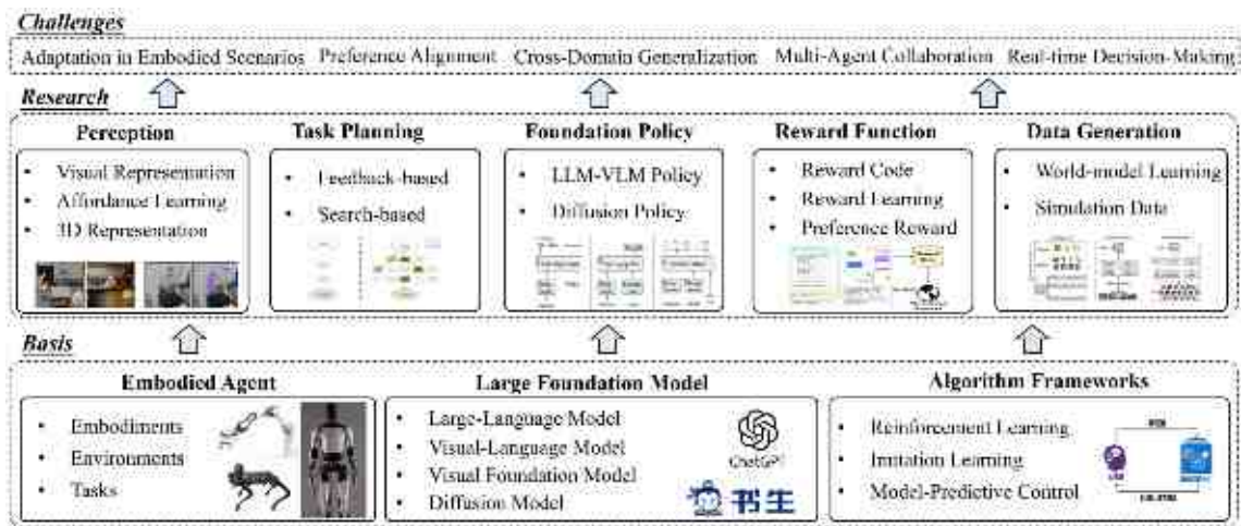
图 2 (网络版彩图) 综述整体框架 Figure 2 (Color online) The overall framework of this survey
